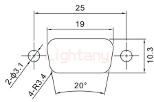
面板开孔 (Panel Cutout)
