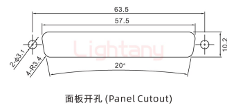
面板开孔 (Panel Cutout)
